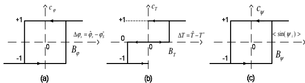
Fig. 5 (a) Flux hysteresis comparator (b) Torque hysteresis comparator (c) Hysteresis comparator of average \sin(\psi_i)
