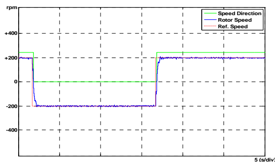
Fig. 16 Rotor speed in the forward and reverse directions
