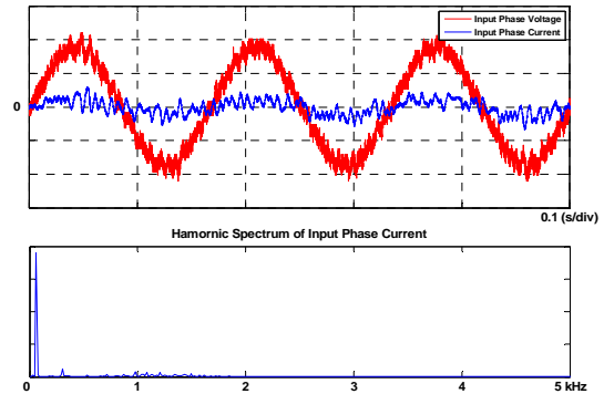
Fig. 17 Input line to neutral voltage (100V/div) and input line current (10A/div) waveforms with 3.5 Nm torque command
