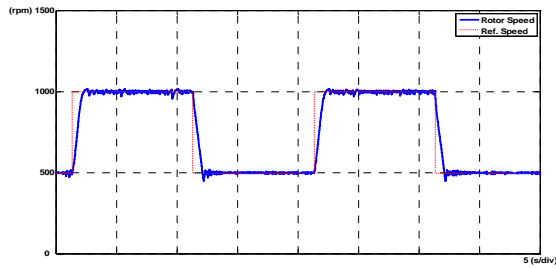
Fig. 13 Rotor speed as the reference speed change from 500 rpm to 1000 rpm with 1 Nm
