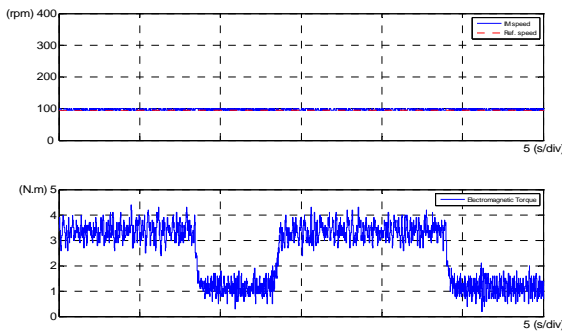
Fig. 15 Electromagnetic torque with the load torque command between 3.5 Nm and 1 Nm
