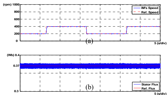
Fig. 12 (a) Rotor speed (b) Stator flux magnitude with the speed command between 200rpm and 400rpm with 1Nm
