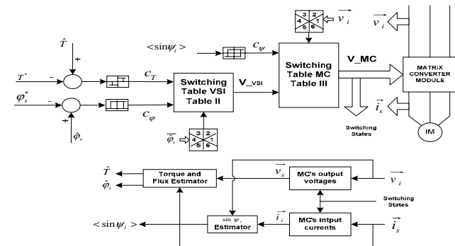
Fig. 6 Block diagram of the DTC with MC
